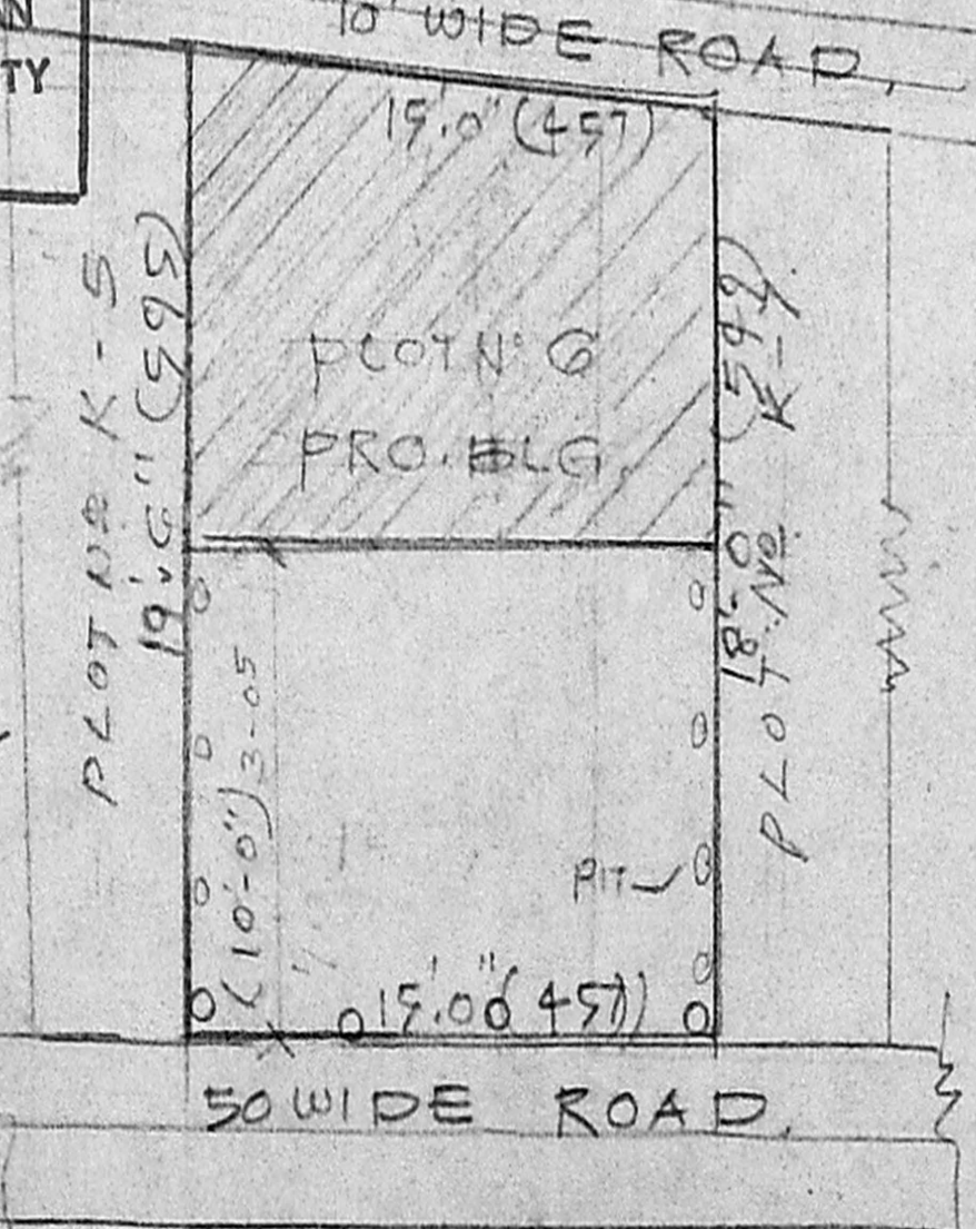
SITE PLAN
